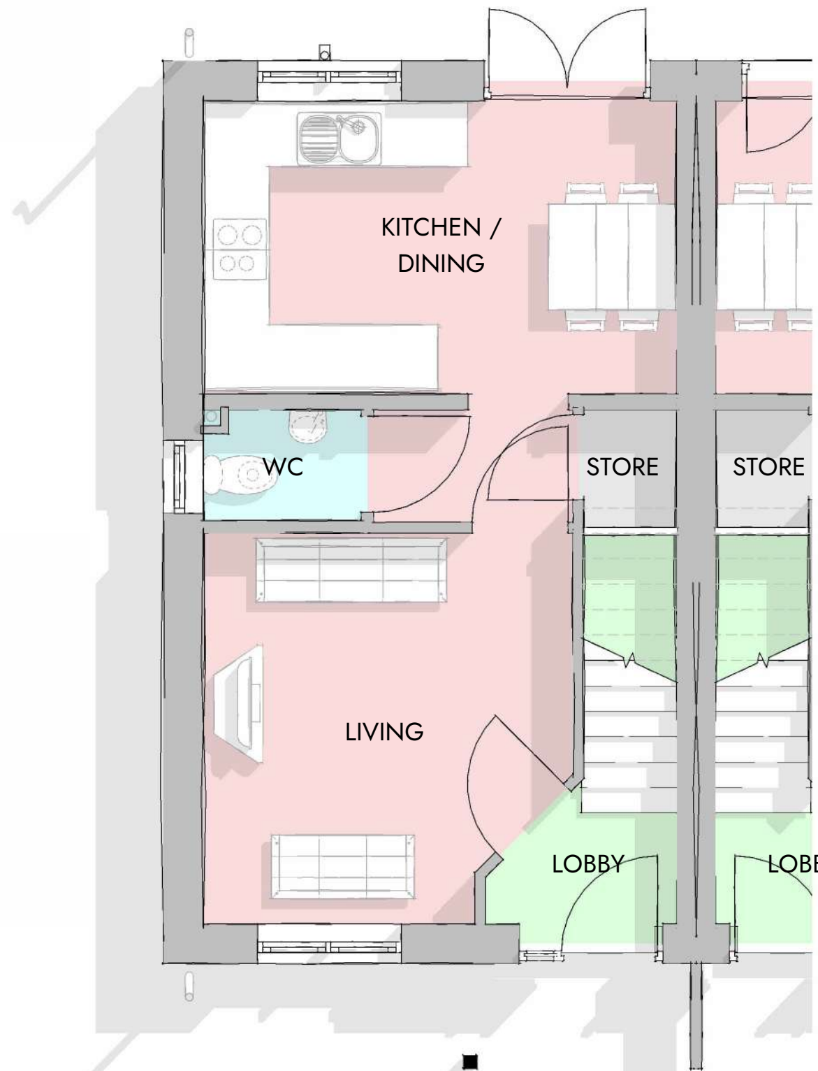
Ground Floor (Handed)
